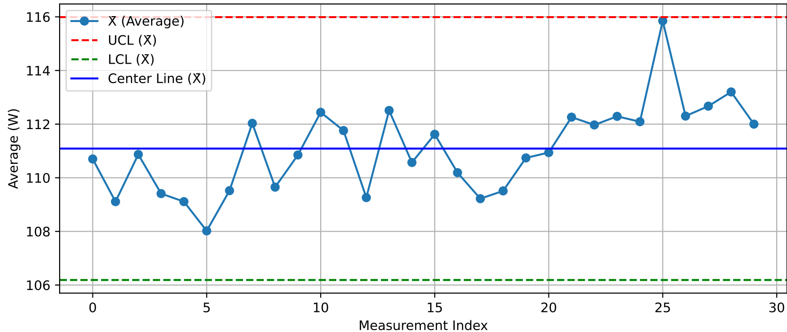
DUT - \bar{X} Chart (T17_Test100@Test.xlsx)
