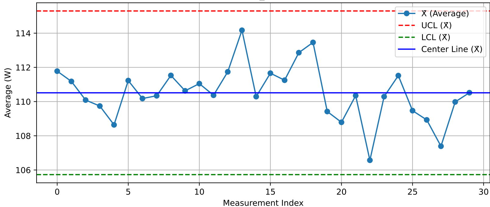
DUT - \bar{X} Chart (T17_Test103@Test.xlsx)
