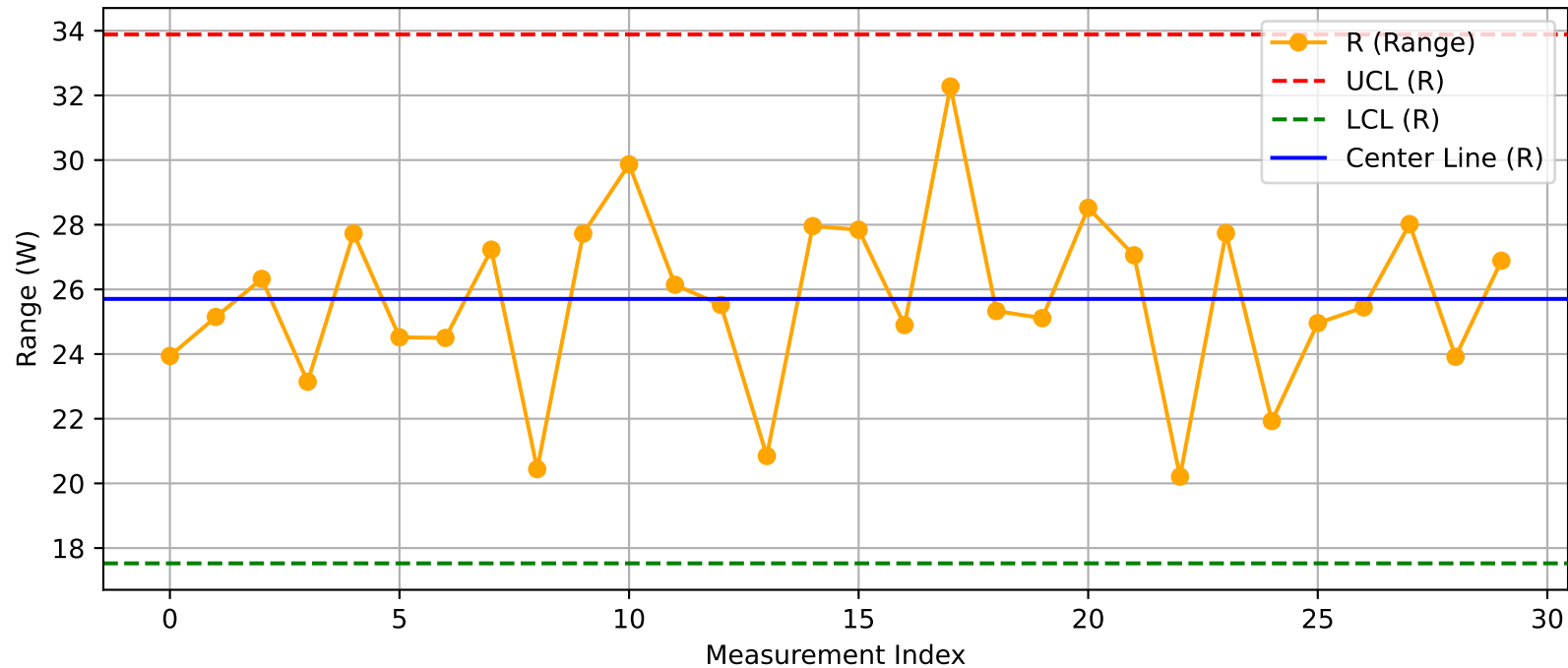
DUT - R Chart (T17_Test203@Test.xlsx)
