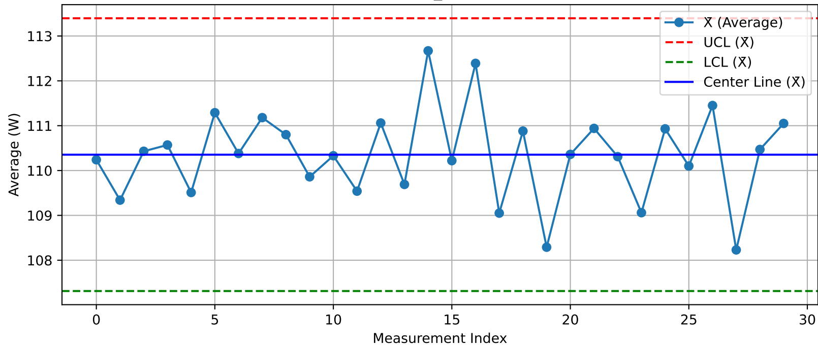
DUT - \bar{X} Chart (T17_Test2O3@Test.xlsx)
