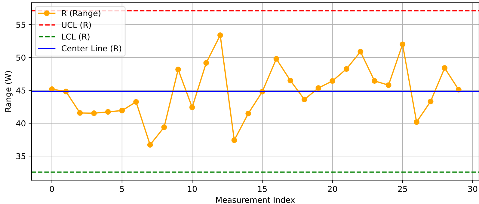
DUT - R Chart (T20_Test100@Test.xlsx)
