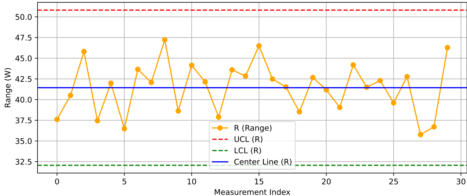
DUT - R Chart (T20_Test1O3@Test.xlsx)
