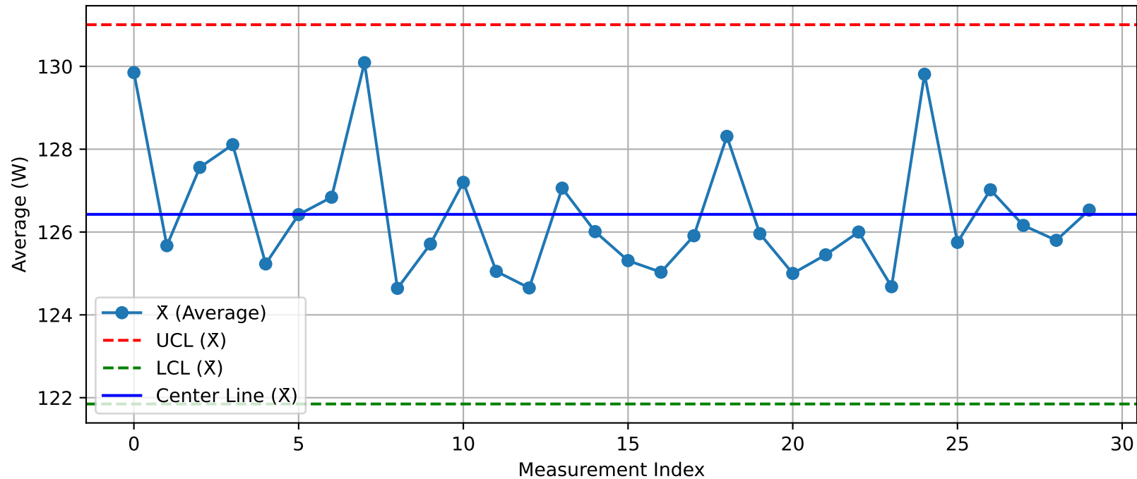
DUT - \bar{X} Chart (T20_Test103@Test.xlsx)
