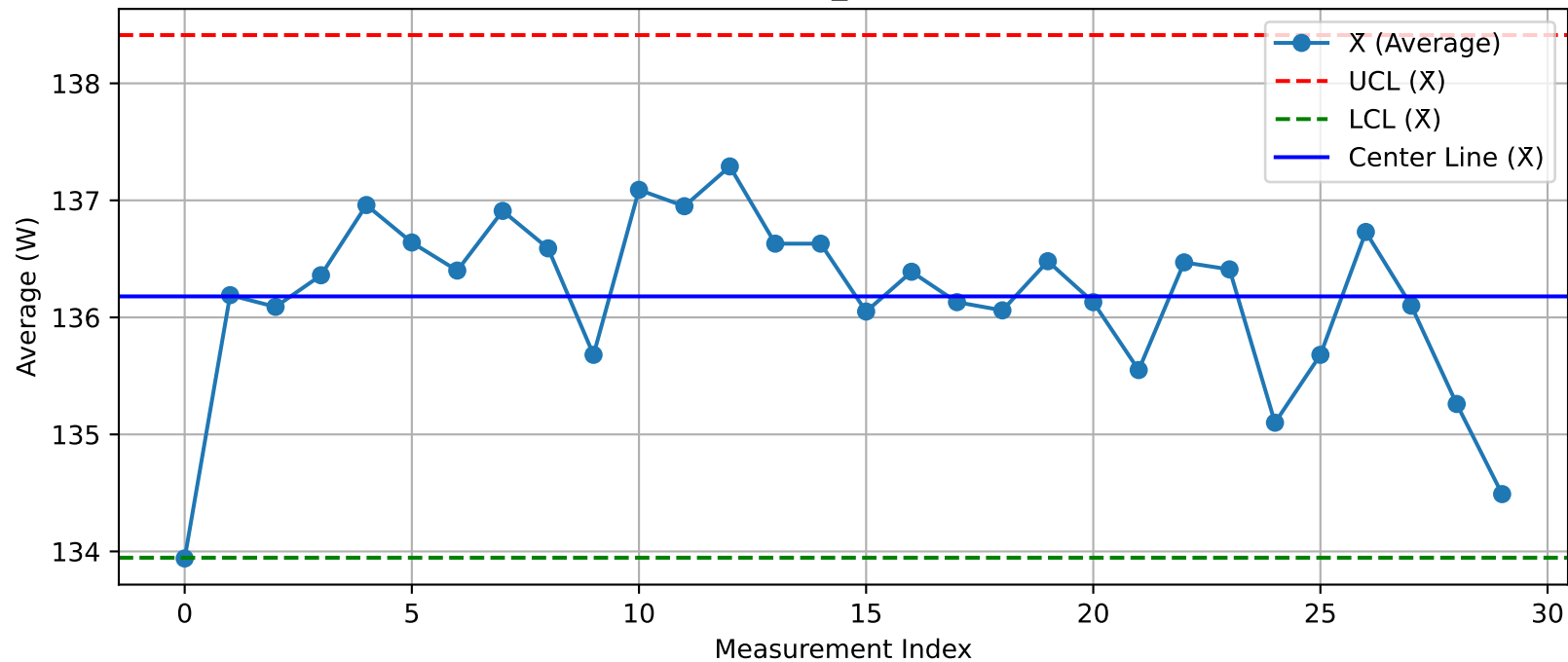
DUT - \bar{X} Chart (T25_Test100@Test.xlsx)
