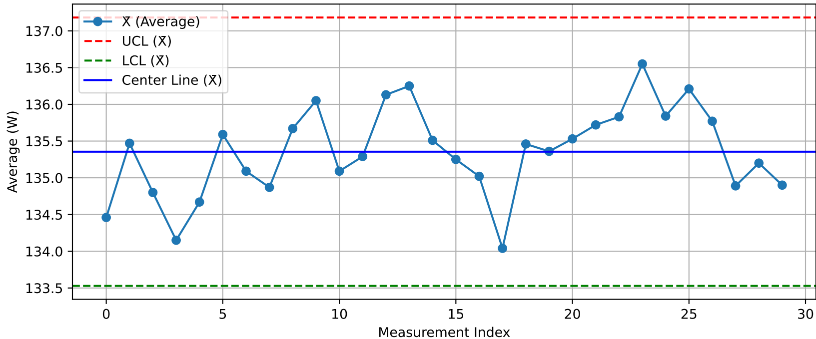
DUT - \bar{X} Chart (T25_Test200@Test.xlsx)
