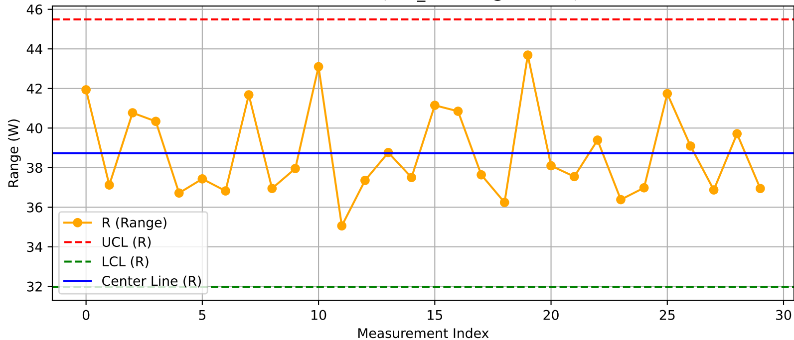
DUT - R Chart (T25_Test203@Test.xlsx)
