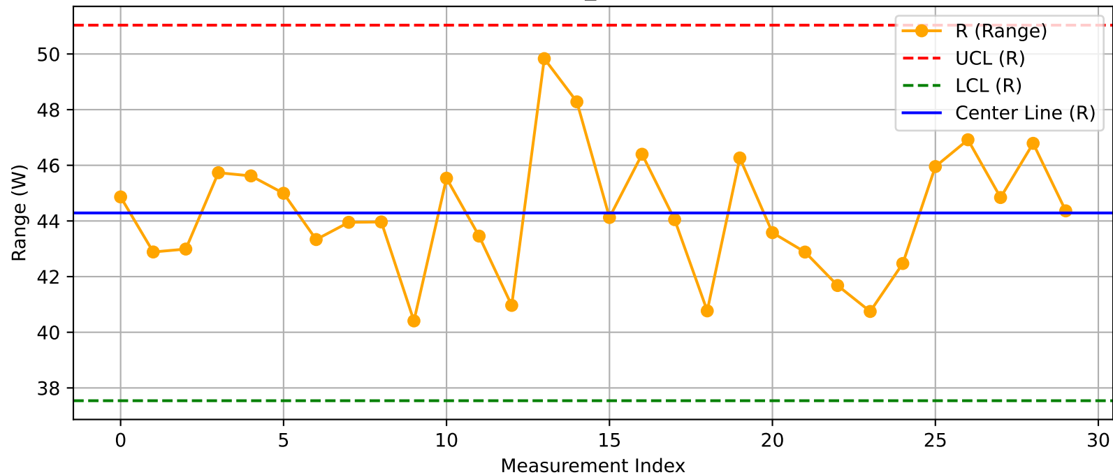
DUT - R Chart (T26_Test100@Test.xlsx)
