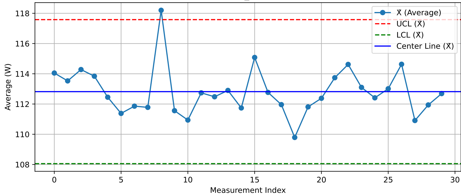
DUT - \bar{X} Chart (T26_Test203@Test.xlsx)
