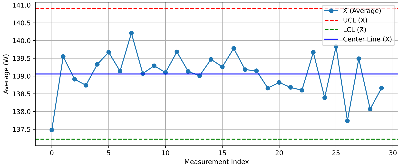
DUT - \bar{X} Chart (T28_Test200@Test.xlsx)
