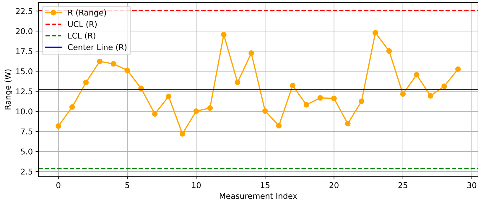
DUT - R Chart (T29_Test100@Test.xlsx)
