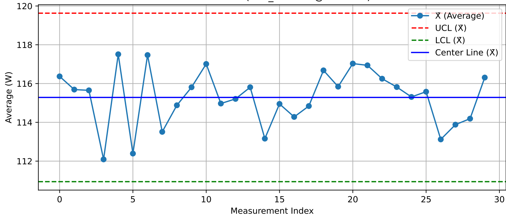
DUT - \bar{X} Chart (T29_Test203@Test.xlsx)
