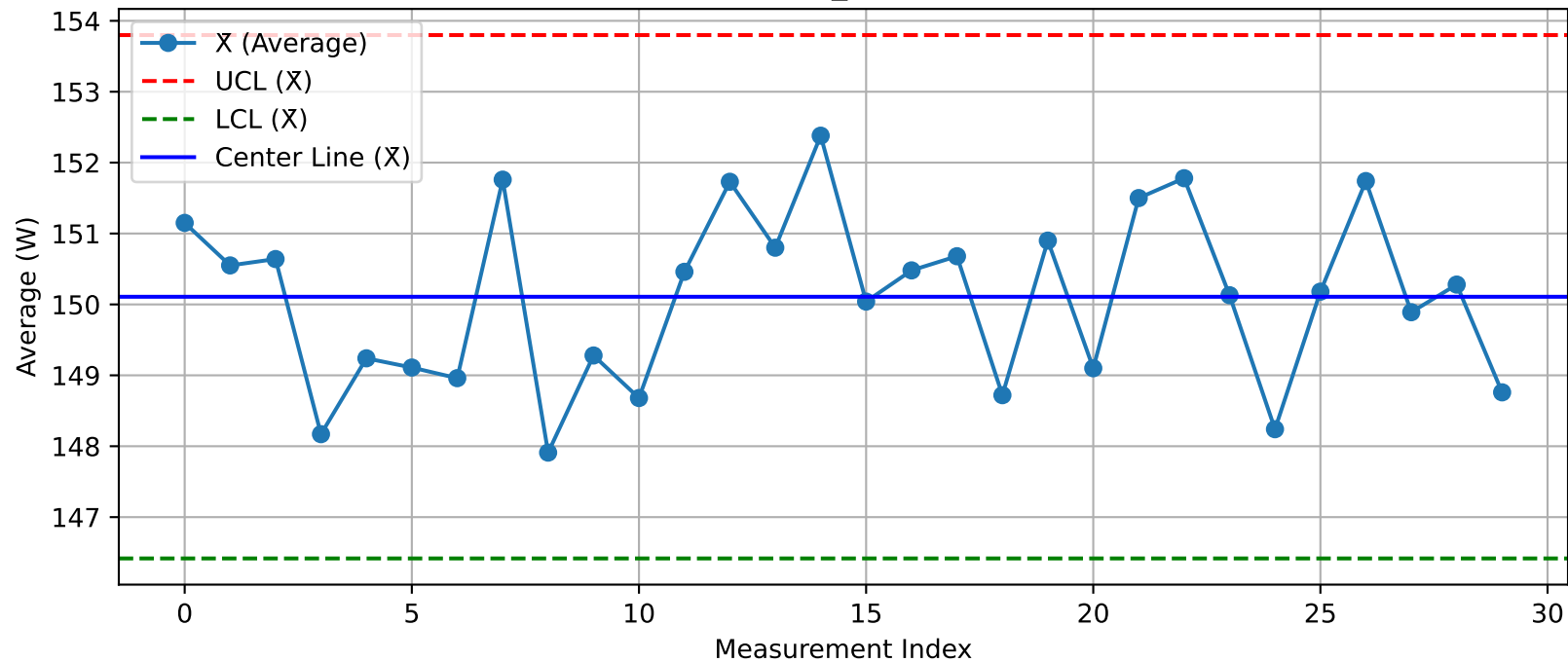
DUT - \bar{X} Chart (T31_Test103@Test.xlsx)
