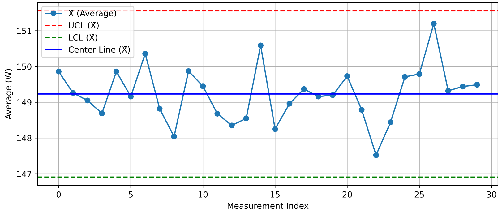
DUT - \bar{X} Chart (T31_Test203@Test.xlsx)
