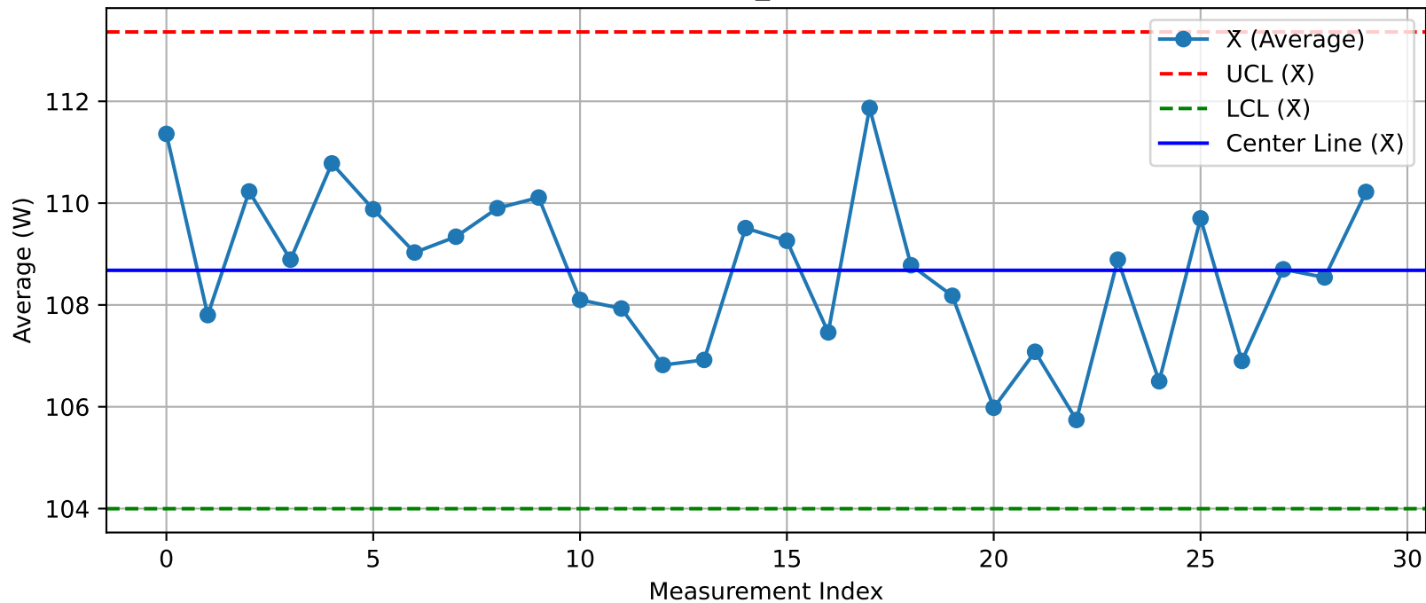
DUT - \bar{X} Chart (T32_Test100@Test.xlsx)
