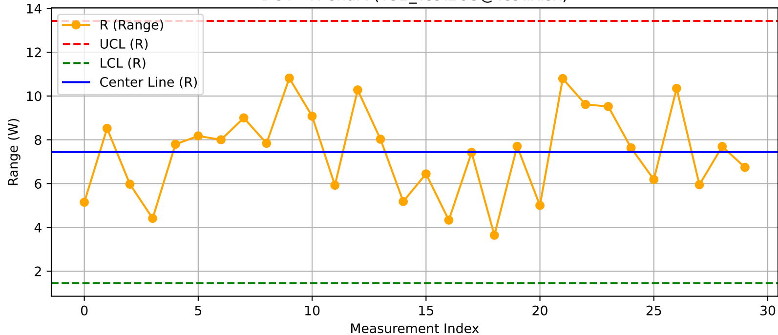
DUT - R Chart (T32_Test203@Test.xlsx)
