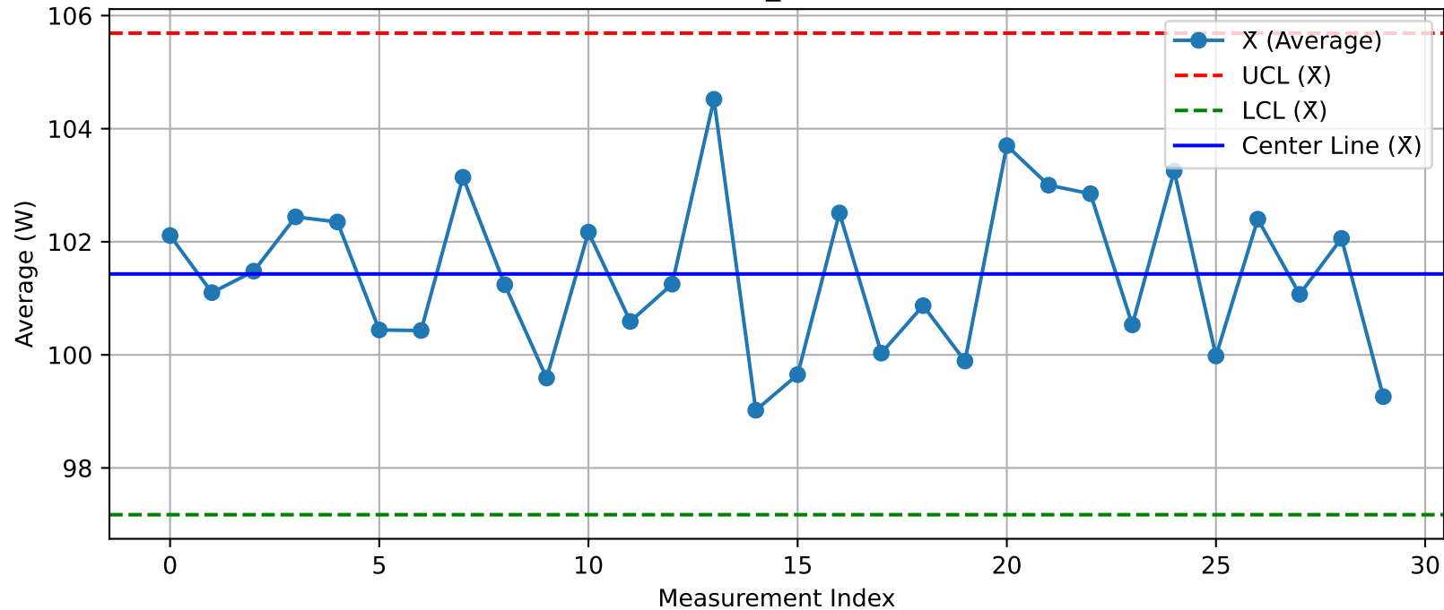
DUT - \bar{X} Chart (T32_Test203@Test.xlsx)
