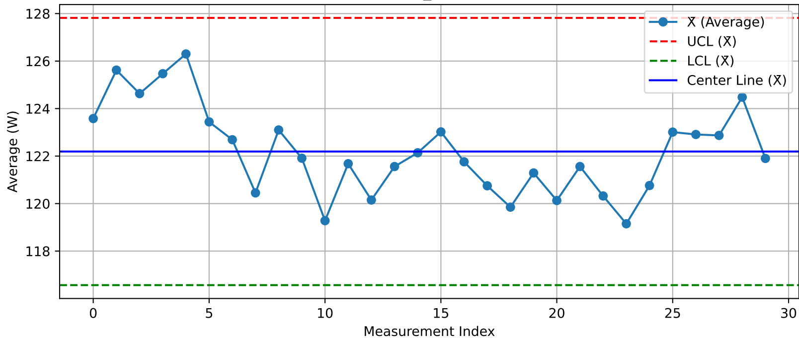
DUT - \bar{X} Chart (T33_Test103@Test.xlsx)
