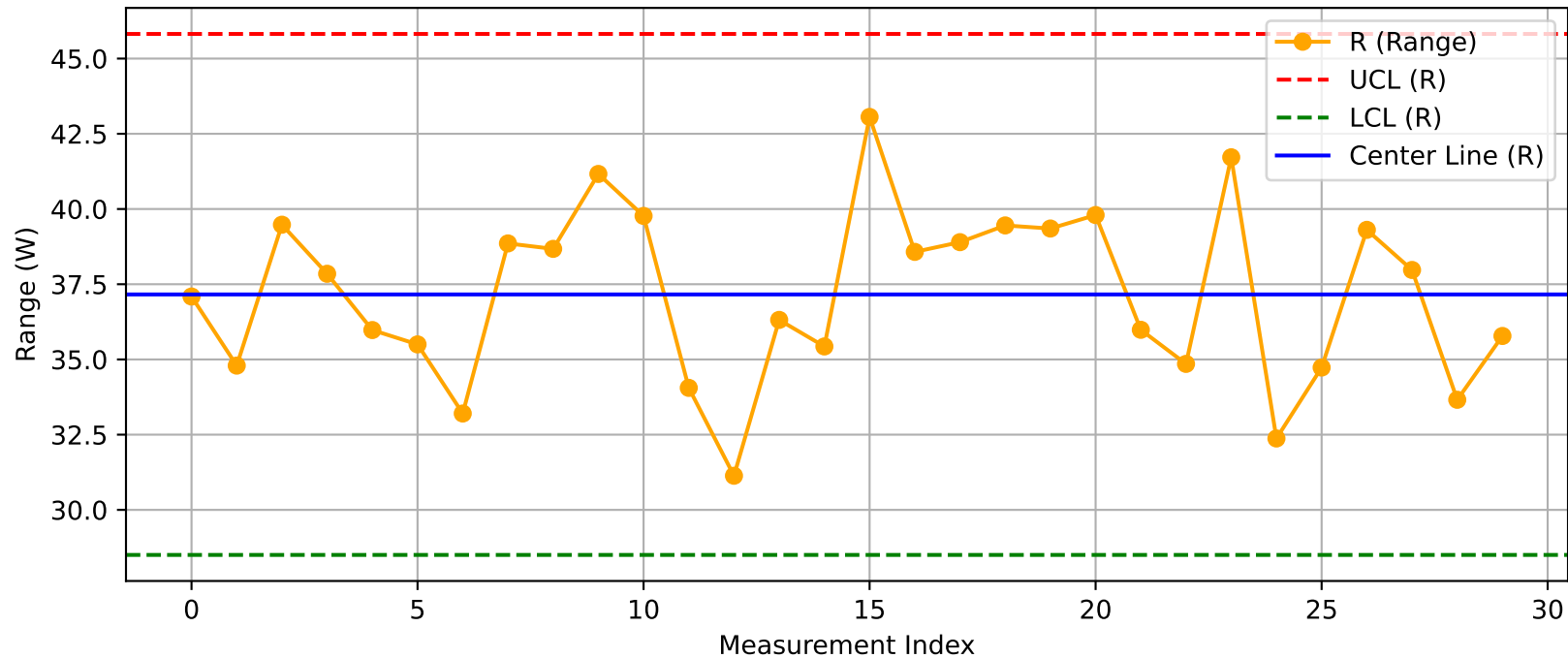
DUT - R Chart (T33_Test200@Test.xlsx)
