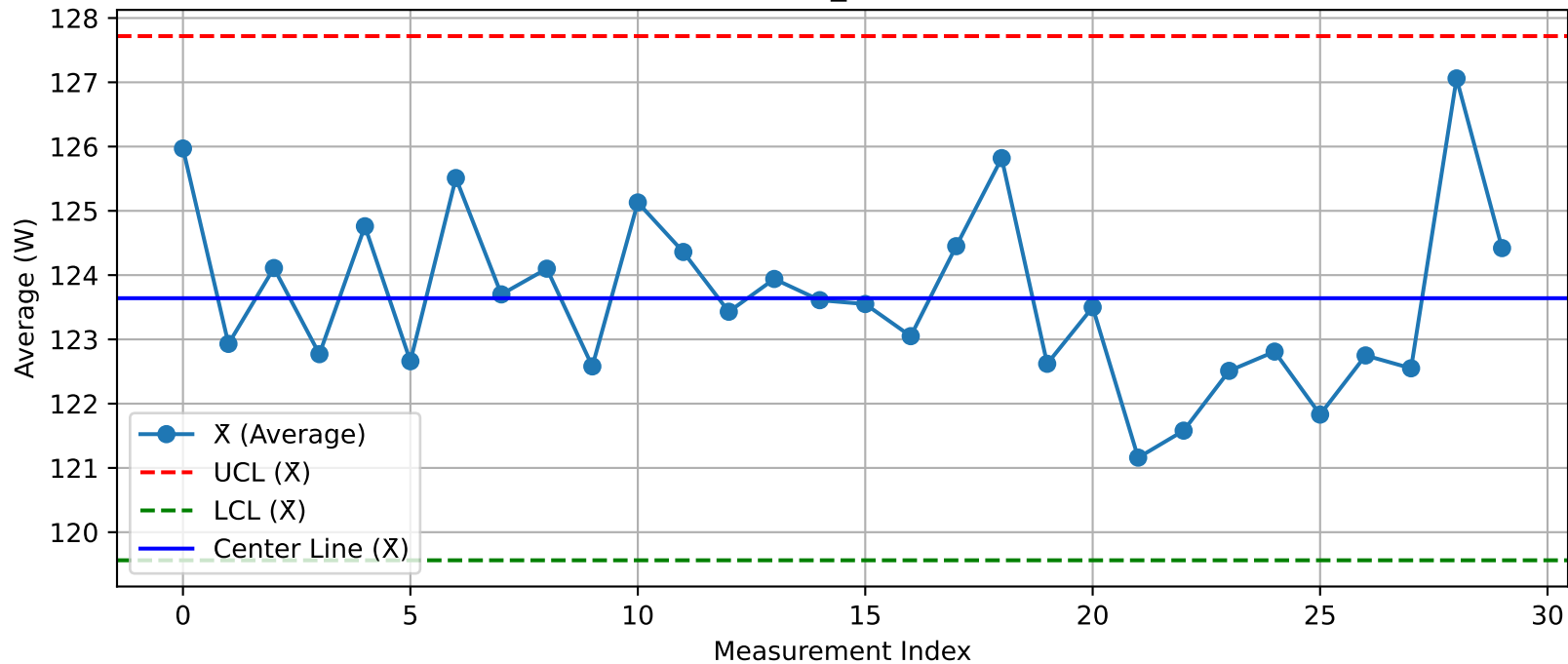
DUT - \bar{X} Chart (T33_Test203@Test.xlsx)
