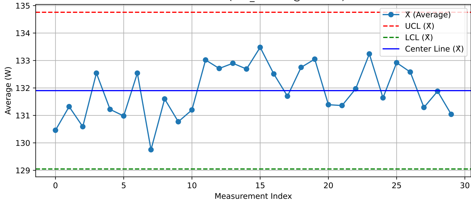
DUT - \bar{X} Chart (T36_Test100@Test.xlsx)
