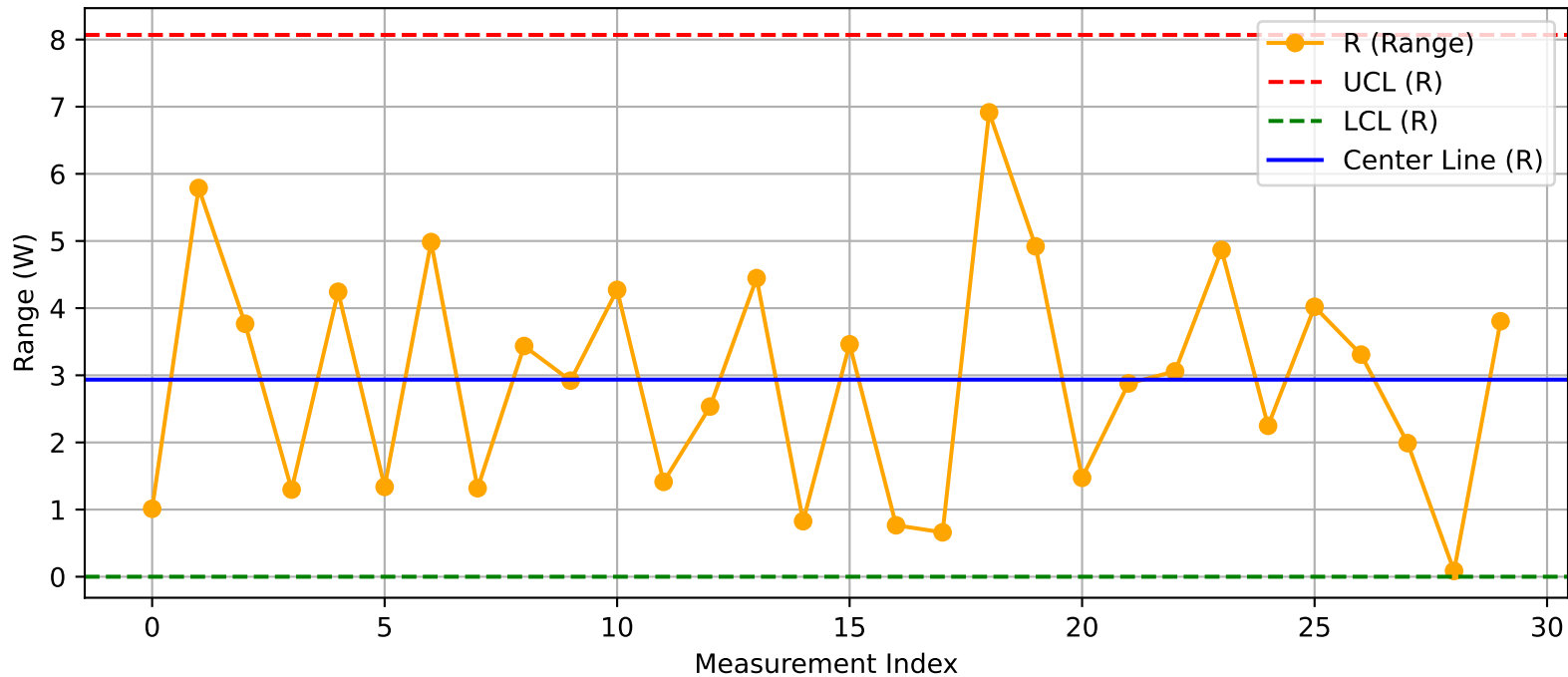
DUT - R Chart (T36_Test203@Test.xlsx)
