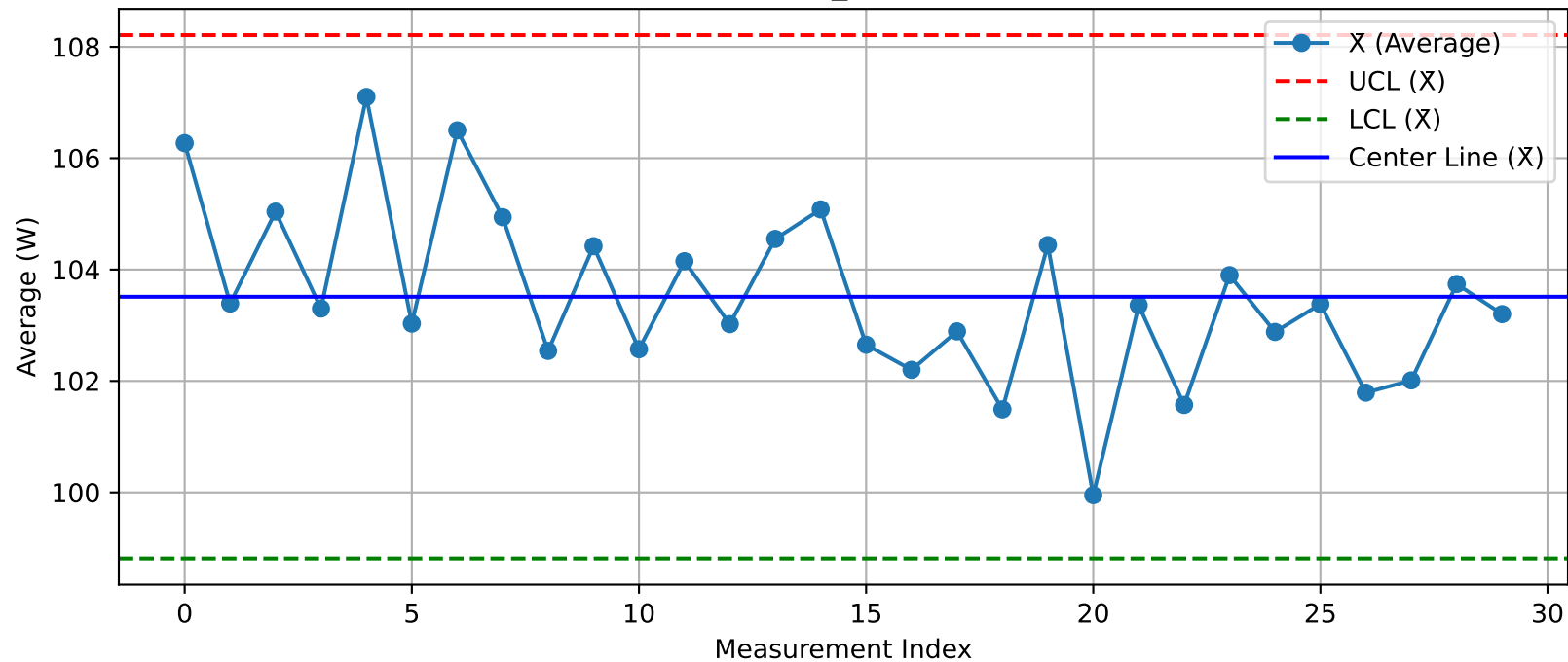
DUT - \bar{X} Chart (T36_Test203@Test.xlsx)
