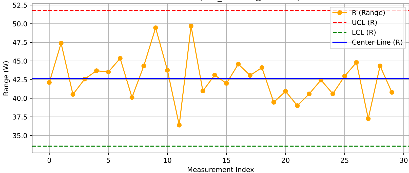
DUT - R Chart (T40_Test2O3@Test.xlsx)
