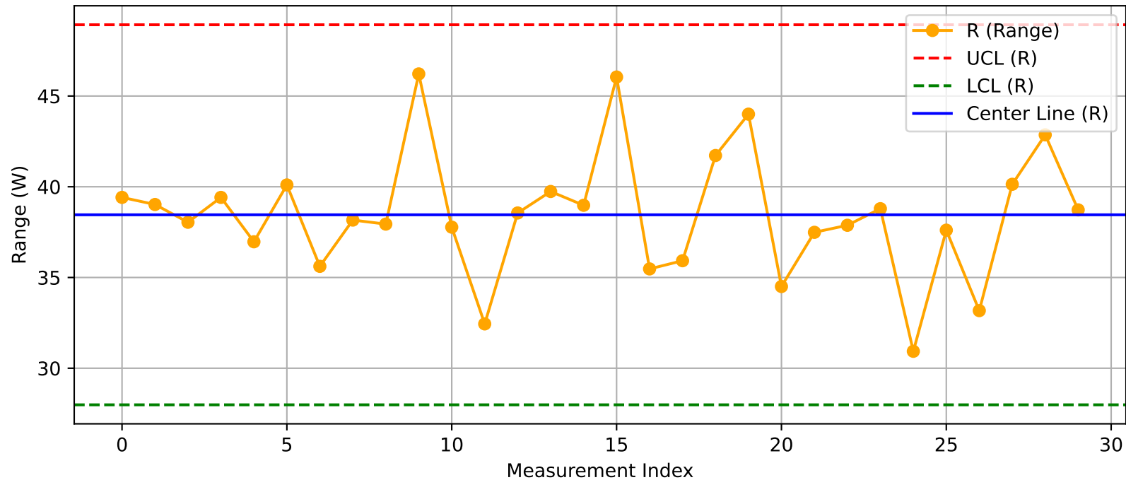
DUT - R Chart (T49_Test2O3@Test.xlsx)
