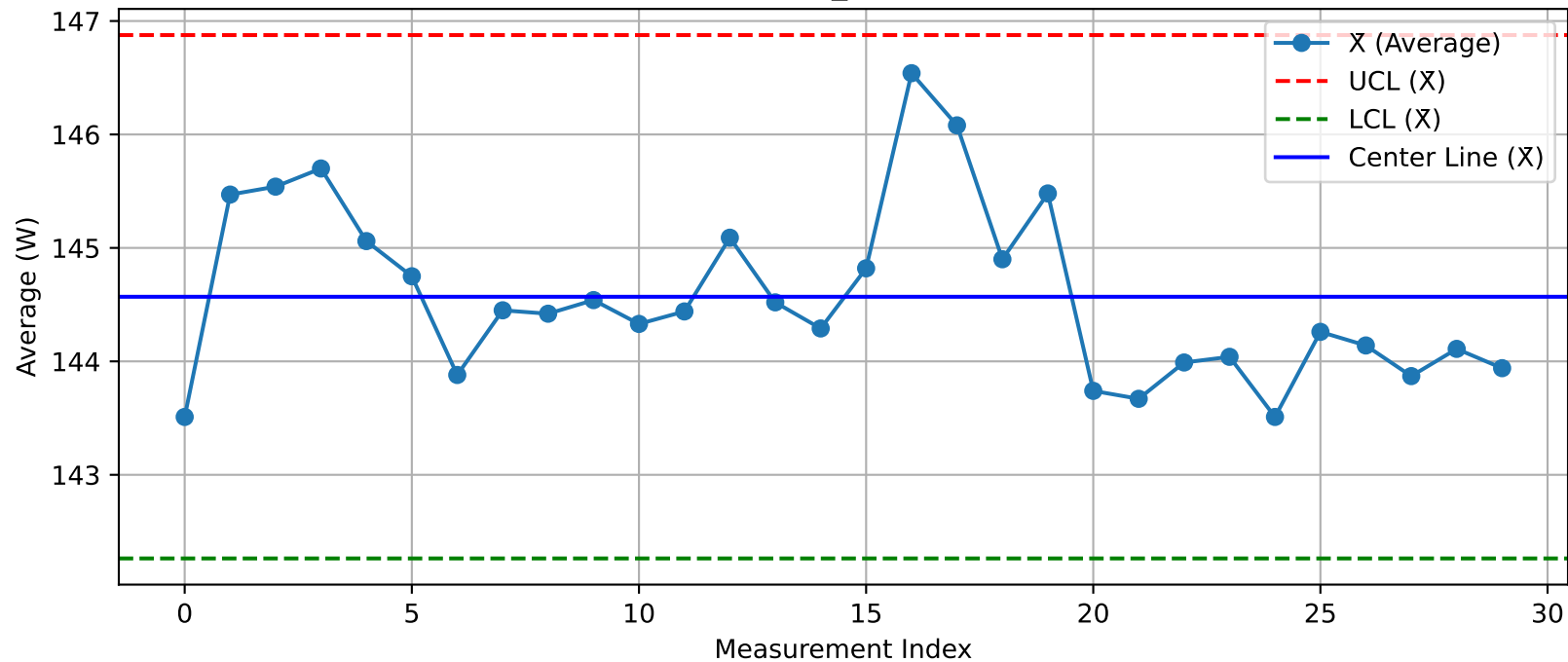
DUT - \bar{X} Chart (T50_Test100@Test.xlsx)
