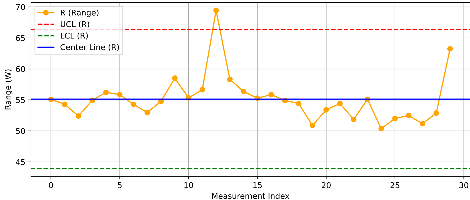
DUT - R Chart (T50_Test200@Test.xlsx)
