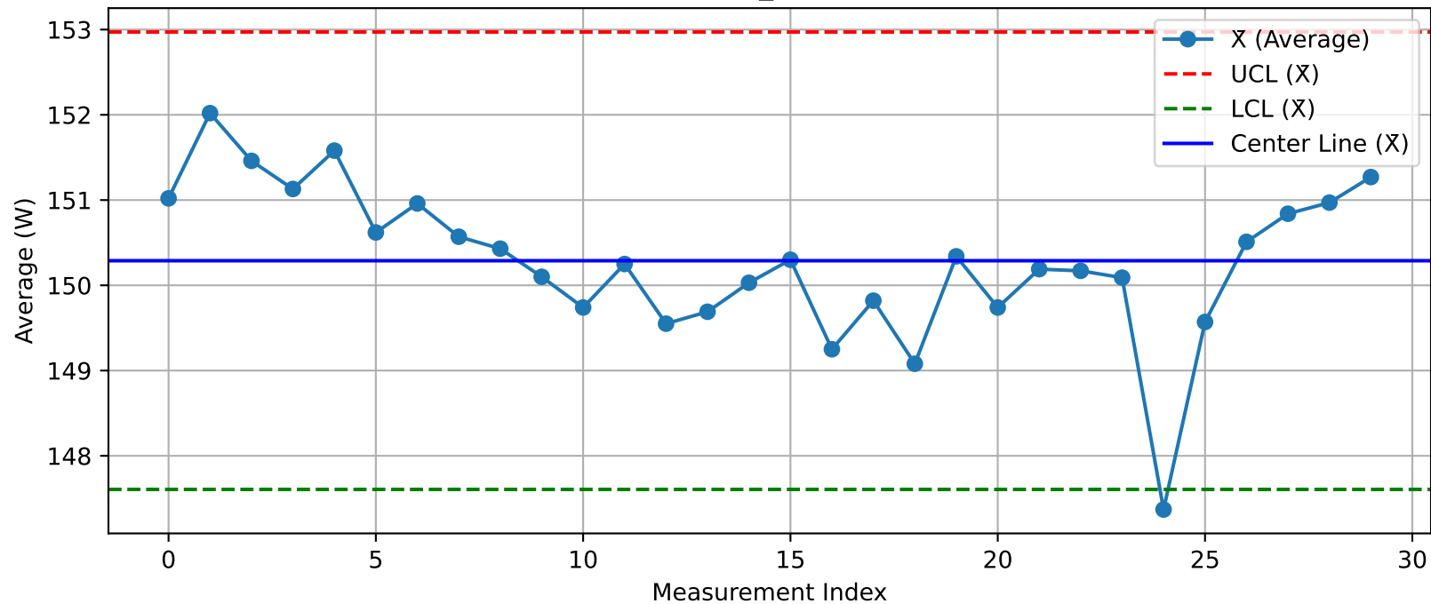
DUT - \bar{X} Chart (T51_Test103@Test.xlsx)
