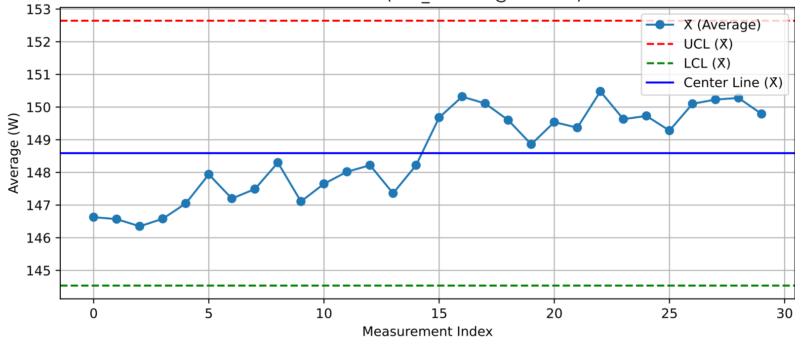
DUT - \bar{X} Chart (T51_Test203@Test.xlsx)
