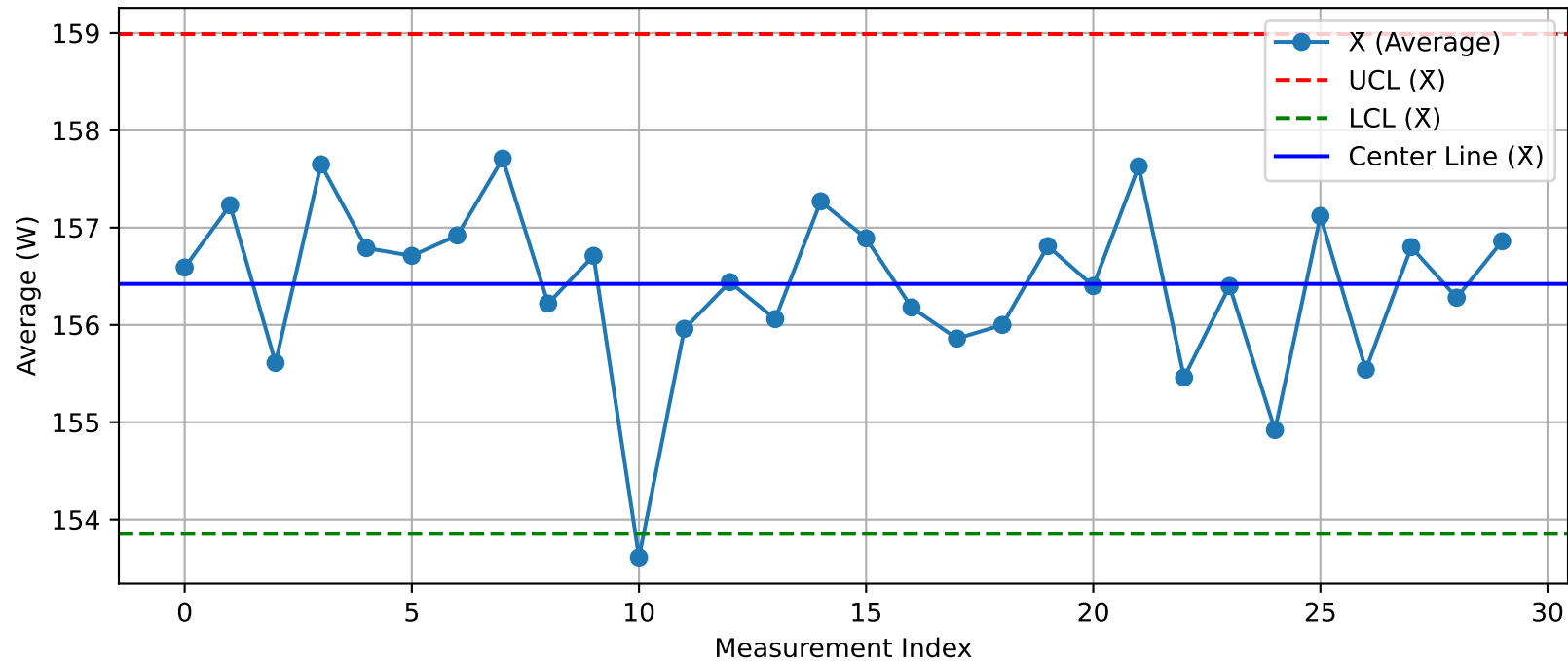
DUT - \bar{X} Chart (T11_Test2_Xint@Test.xlsx)
