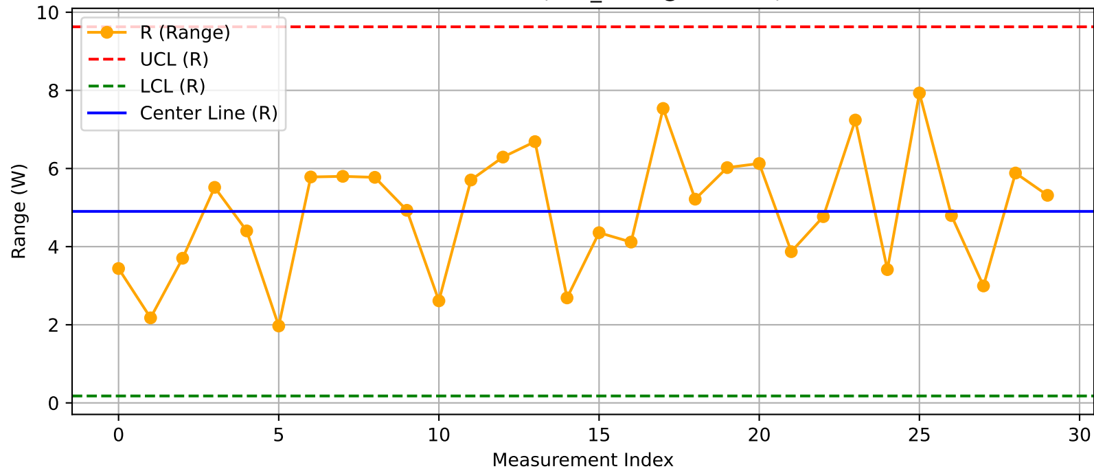
DUT - R Chart (T12_Test1@Test.xlsx)
