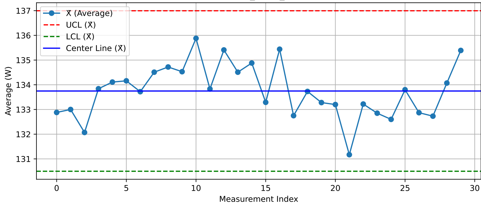
DUT - X Chart (T13_Test1_Xint@Test.xlsx)
