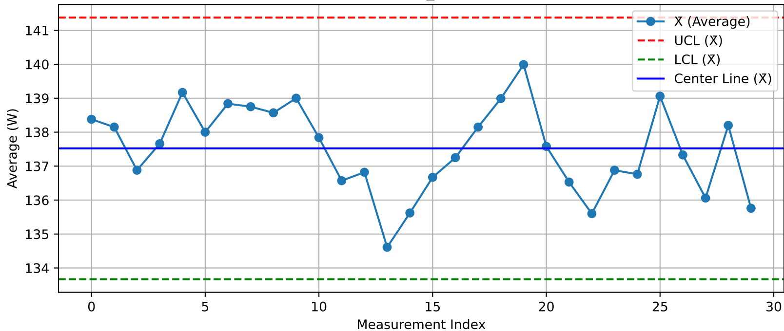
DUT - \bar{X} Chart (T13_Test2@Test.xlsx)
