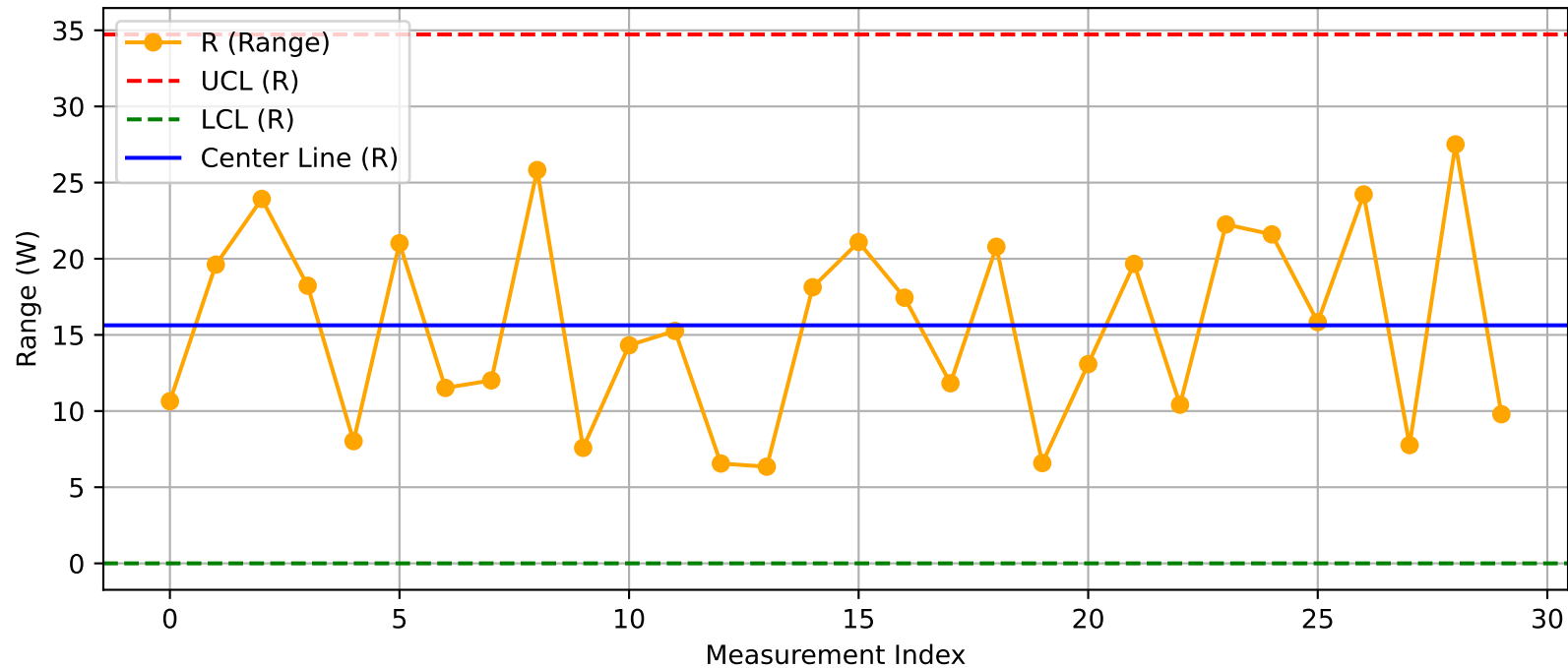
DUT - R Chart (T17_Test1_Xint@Test.xlsx)
