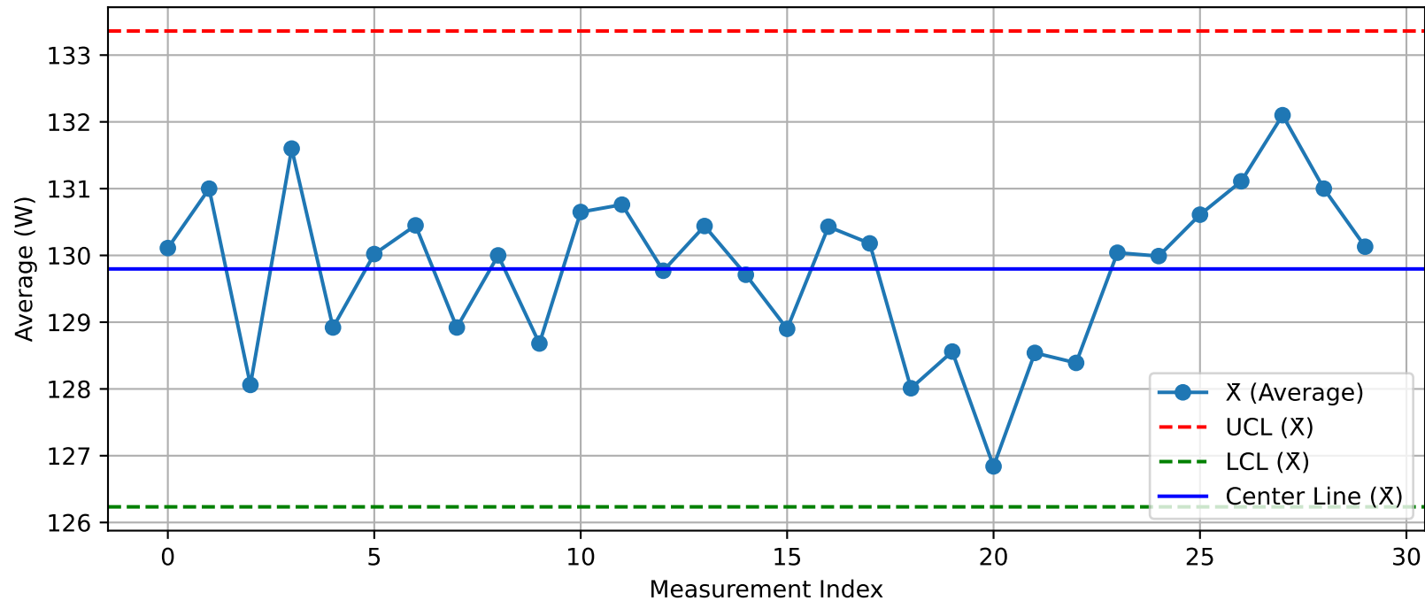
DUT - \bar{X} Chart (T17_Test2_Xint@Test.xlsx)
