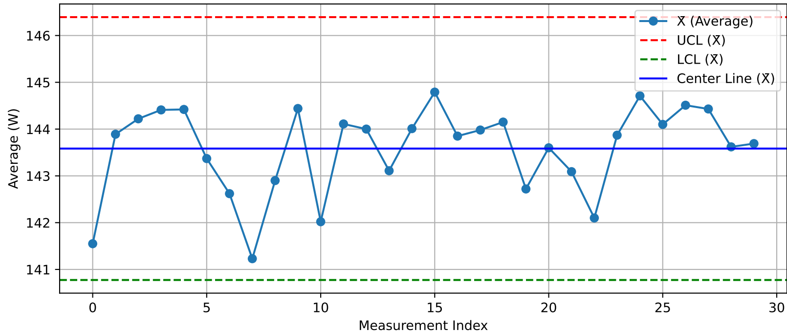
DUT - \bar{X} Chart (T19_Test1_Xint@Test.xlsx)
