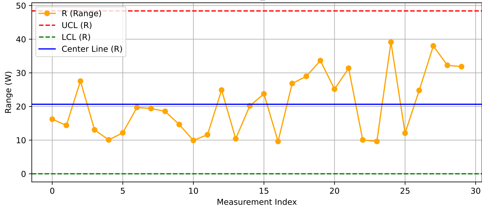
DUT - R Chart (T20_Test1@Test.xlsx)
