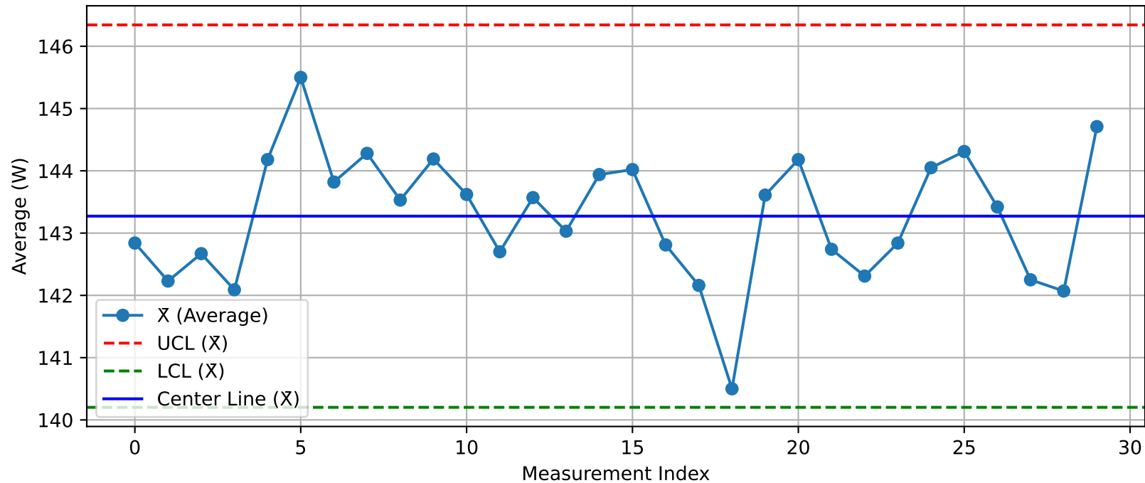
DUT - \bar{X} Chart (T26_Test1_Xint@Test.xlsx)
