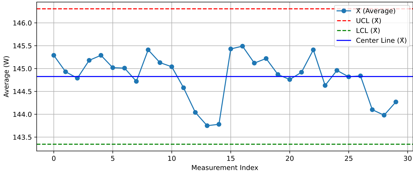
DUT - \bar{X} Chart (T26_Test2_Xint@Test.xlsx)
