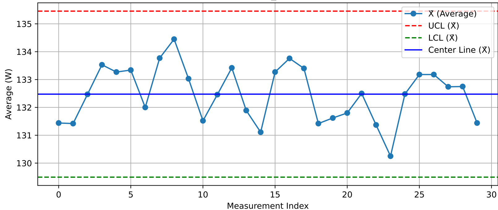
DUT - \bar{X} Chart (T28_Test2@Test.xlsx)
