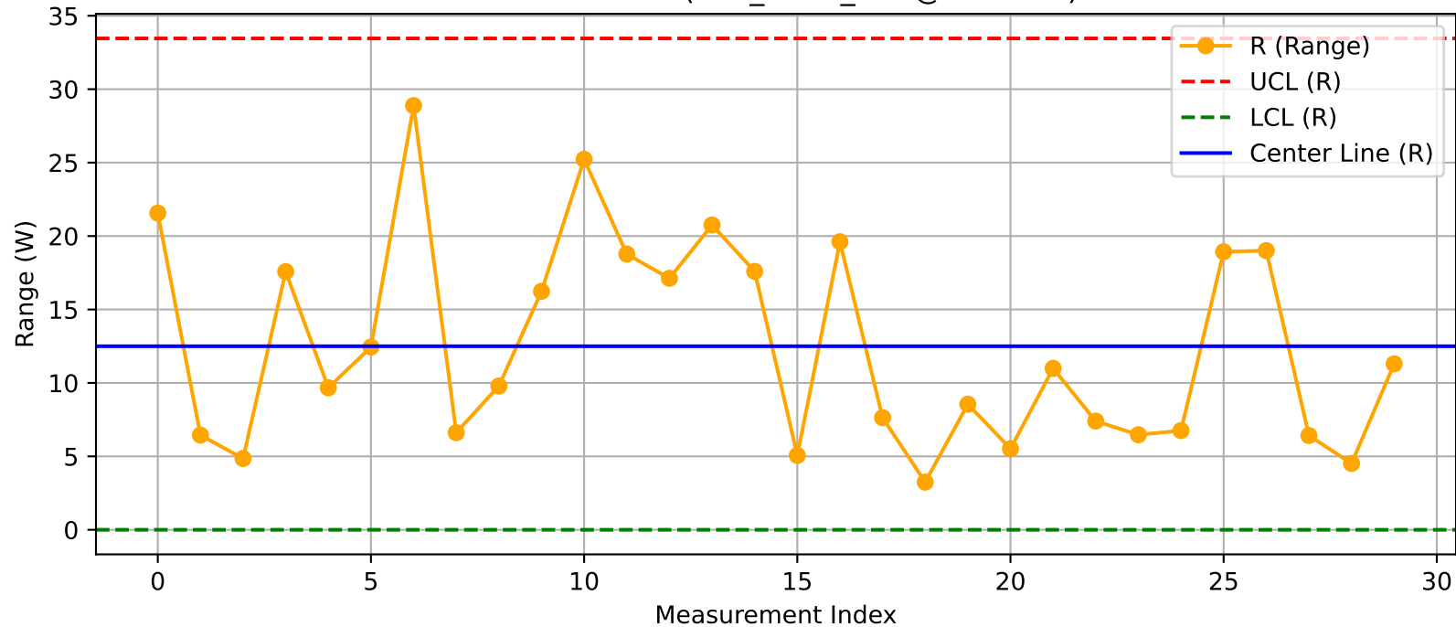
DUT - R Chart (T29_Test2_Xint@Test.xlsx)
