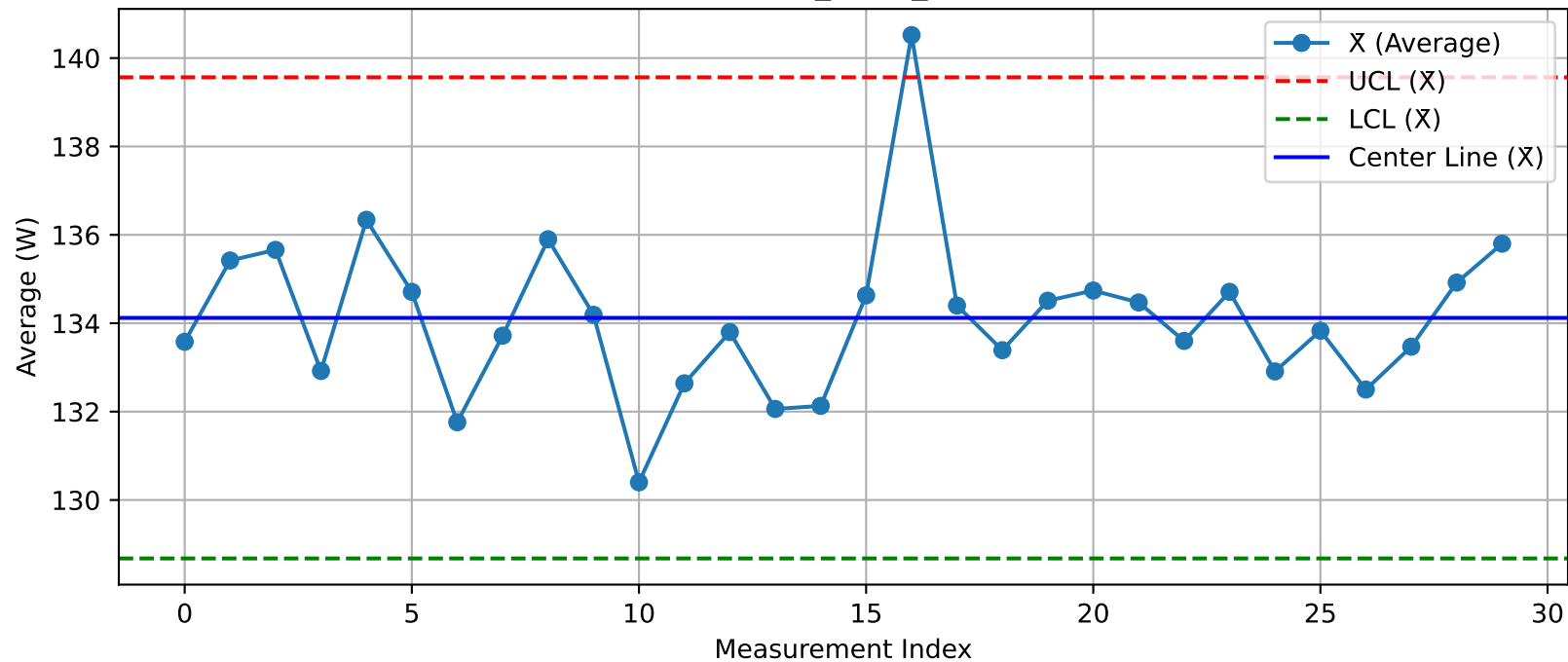
DUT - X Chart (T29_Test2_Xint@Test.xlsx)
