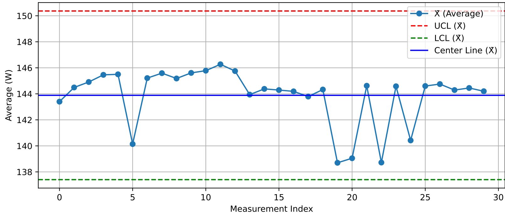
DUT - \bar{X} Chart (T31_Test1@Test.xlsx)
