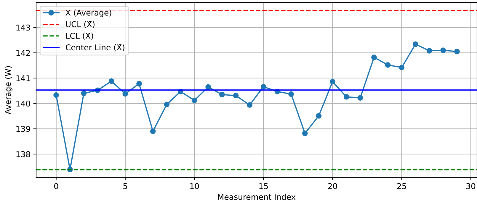
DUT - \bar{X} Chart (T31_Test2_Xint@Test.xlsx)
