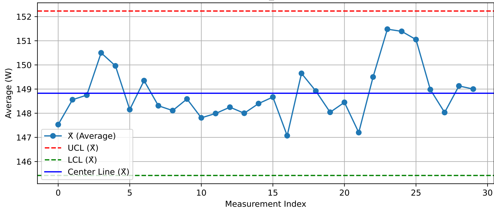
DUT - \bar{X} Chart (T32_Test1@Test.xlsx)
