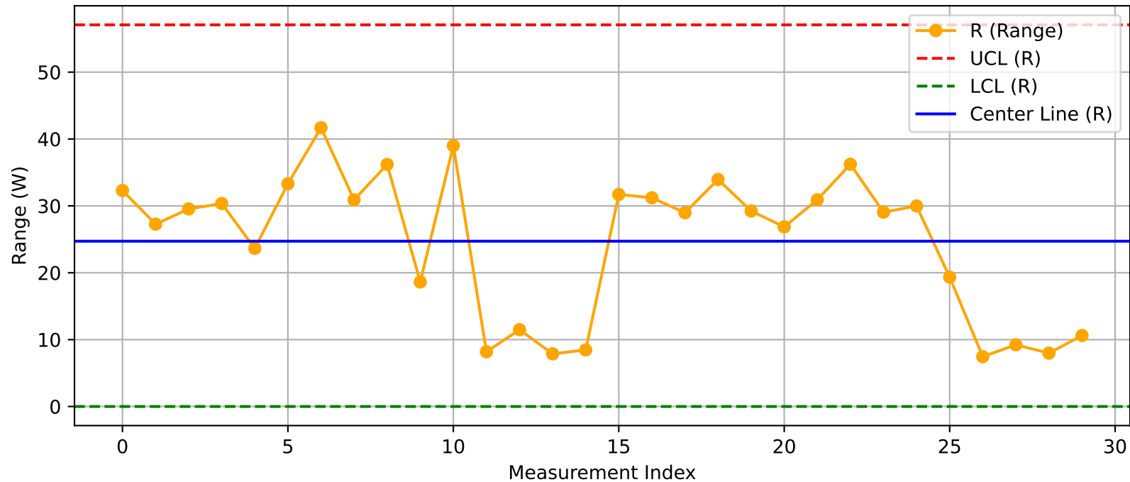
DUT - R Chart (T36_Test1_Xint@Test.xlsx)
