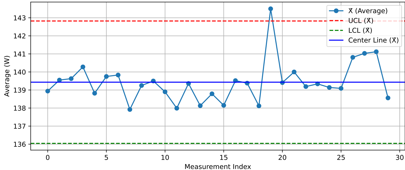
DUT - X Chart (T40_Test2_Xint@Test.xlsx)
